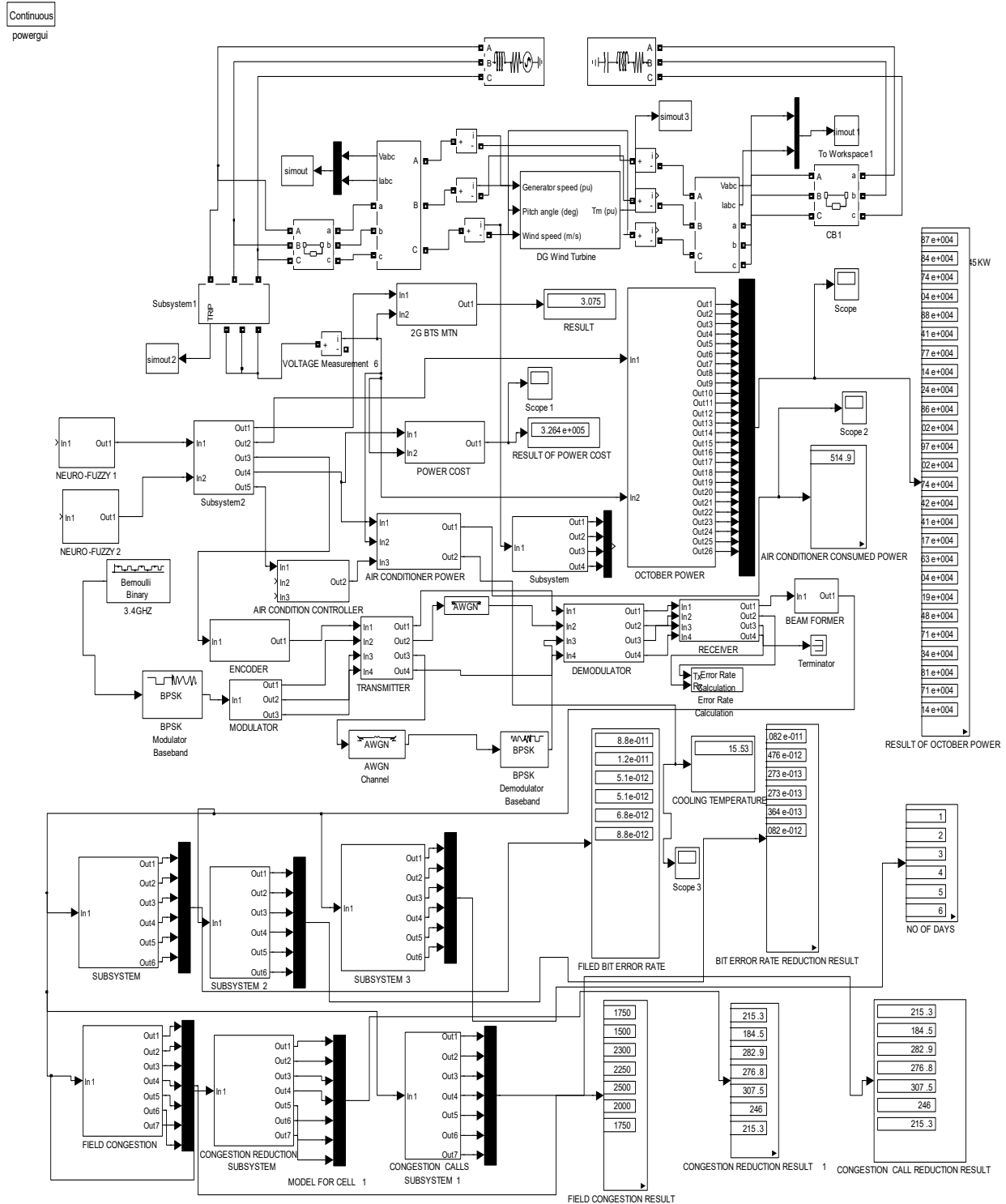
Figure 5: Designed Simulink Model for Improving Energy Efficiency through Reduction of Power Consumption in the Base Station or a Cell Site using Neuro-Fuzzy Controller
