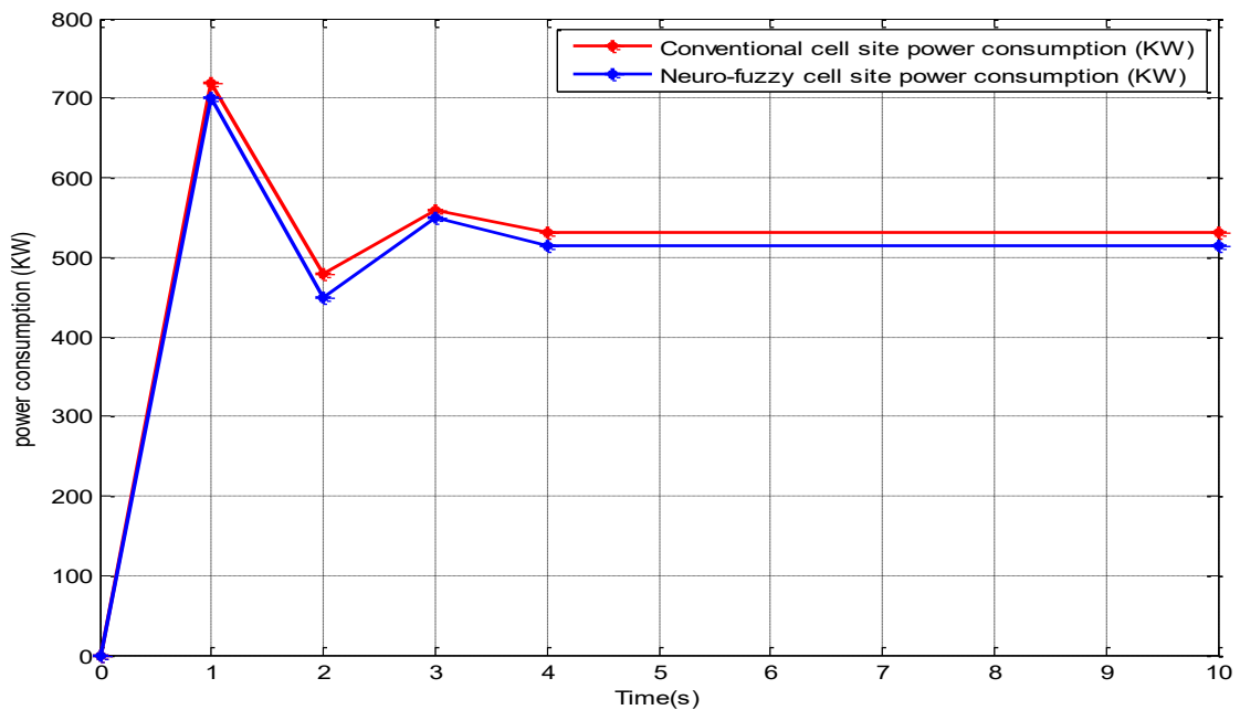
Figure 6: Comparing Power Consumed in the cell site without and with Neuro-Fuzzy Controller
